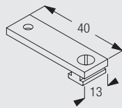
6138p Ceiling Support
