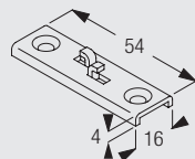
6124 Bracket
