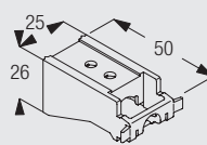
3655 Bracket
