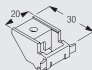
3603 Bracket
