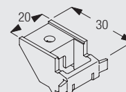
3603 Bracket
